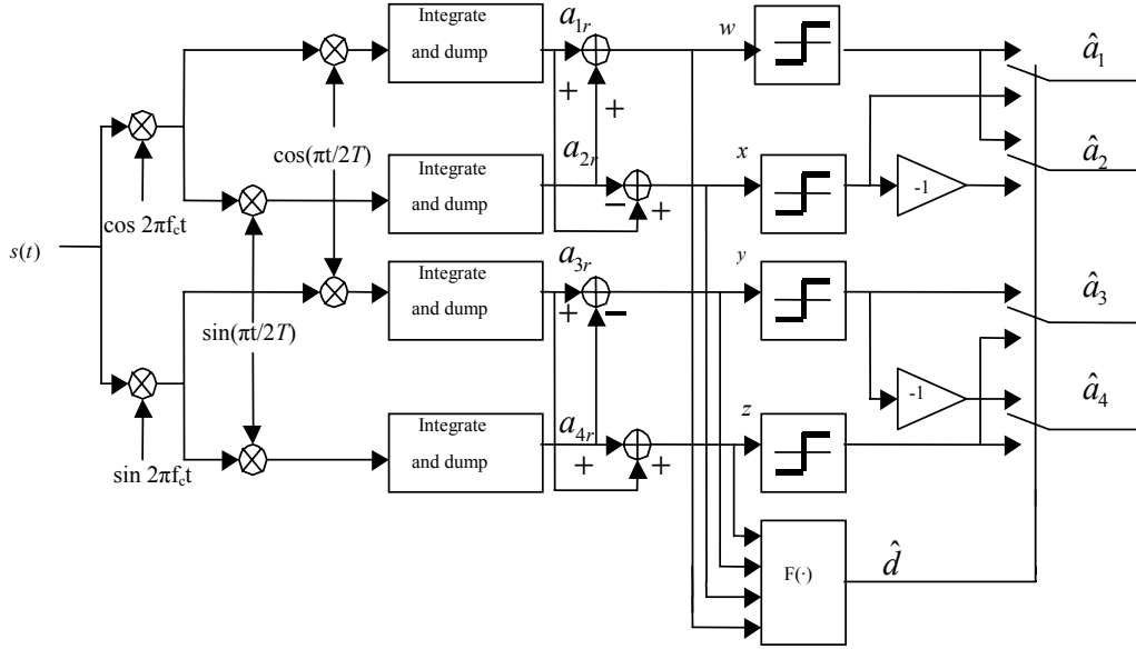
Fig.1. Block diagram of the proposed optimum CEQ 2 PSK demodulator and detector.
